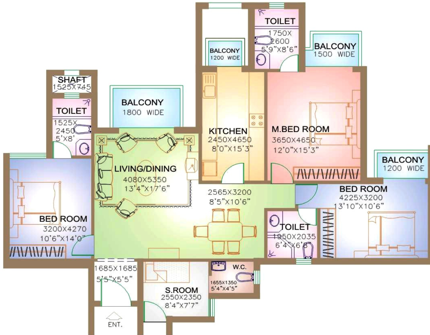
TENTATIVE TYPICAL APARTMENT PLAN
